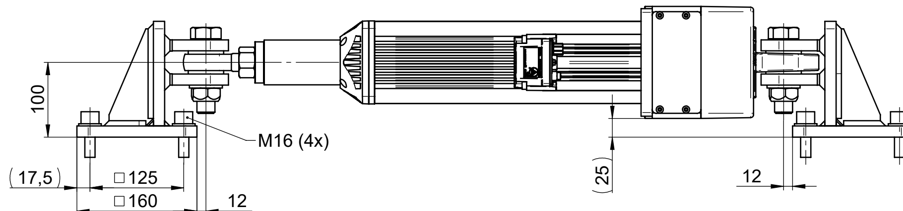
Wandmontage / wall mounting (AG_9809-10665291F)
