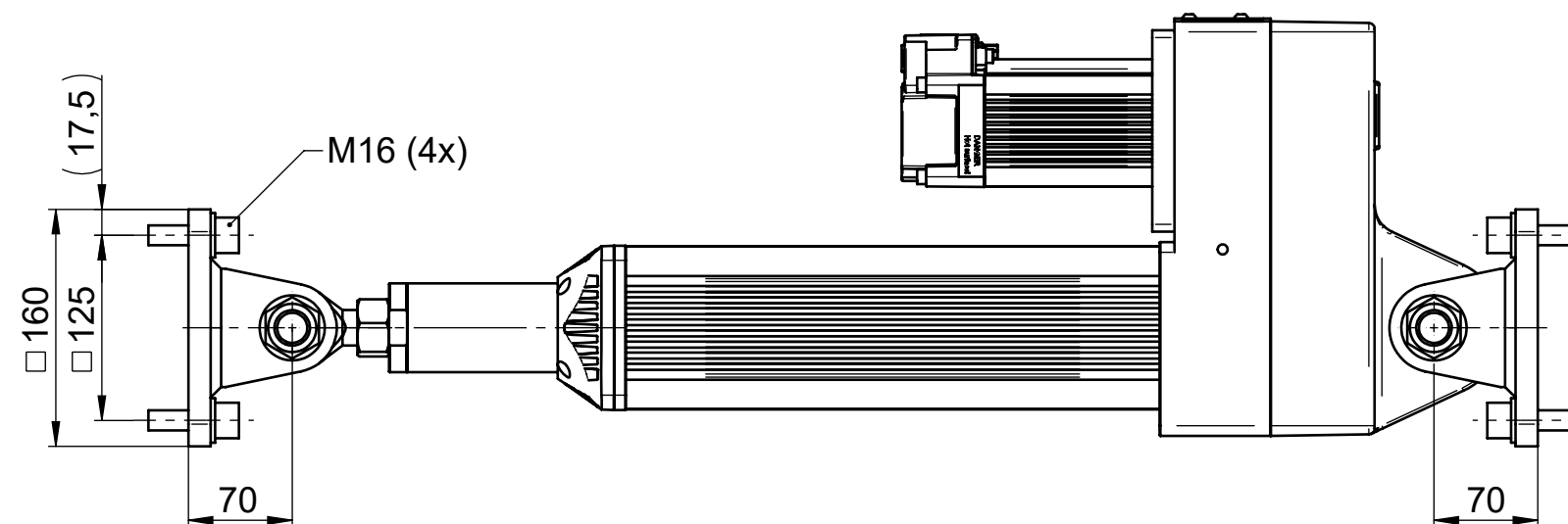
Bodenmontage / floor mounting (AG_9809-10666348F)
