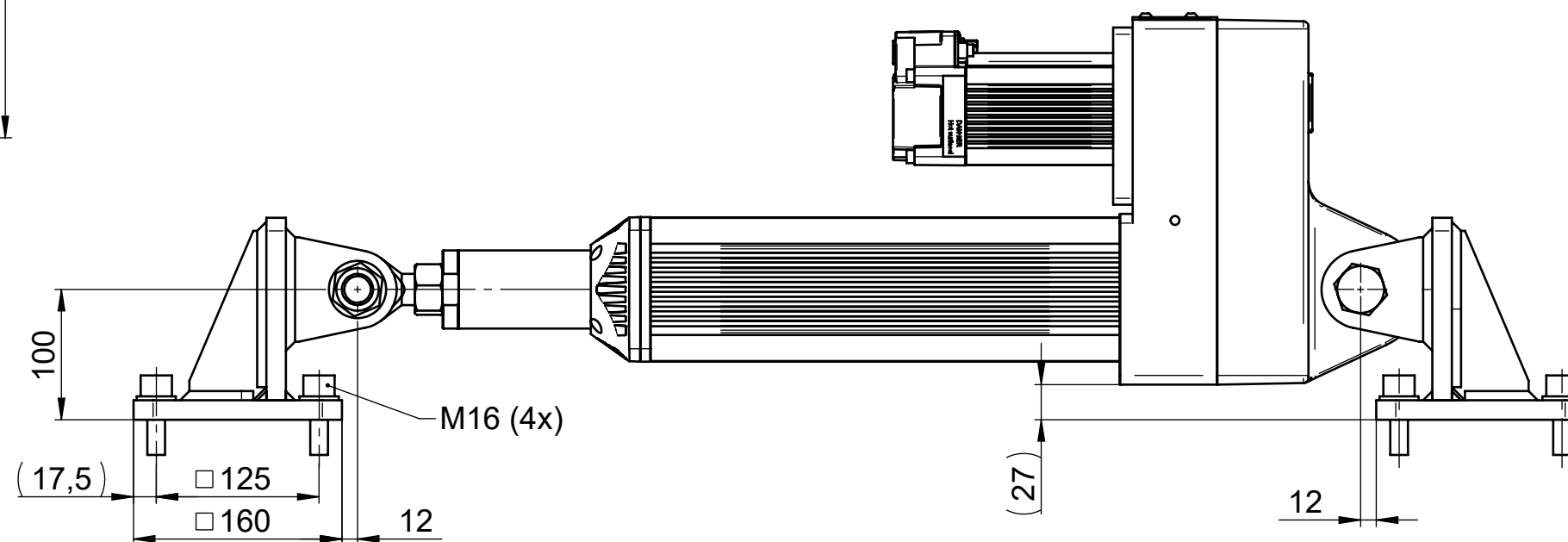
Bodenmontage / floor mounting (AG_9809-10666348F)
